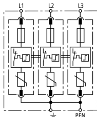
Basic circuit diagram DG M TNC CI 275
