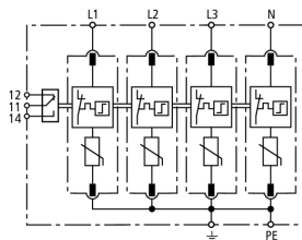
Basic circuit diagram DG M TNS 150 FM
