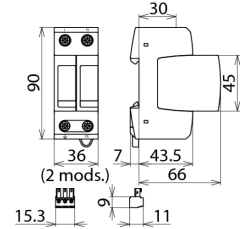
Dimension drawing DG M TN 150 FM
