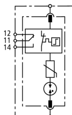
Basic circuit diagram DG S 385 VA FM
