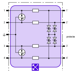
Basic circuit diagram BXT ML4 BC 24
