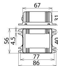
Dimension drawing DLI TC 2 I
